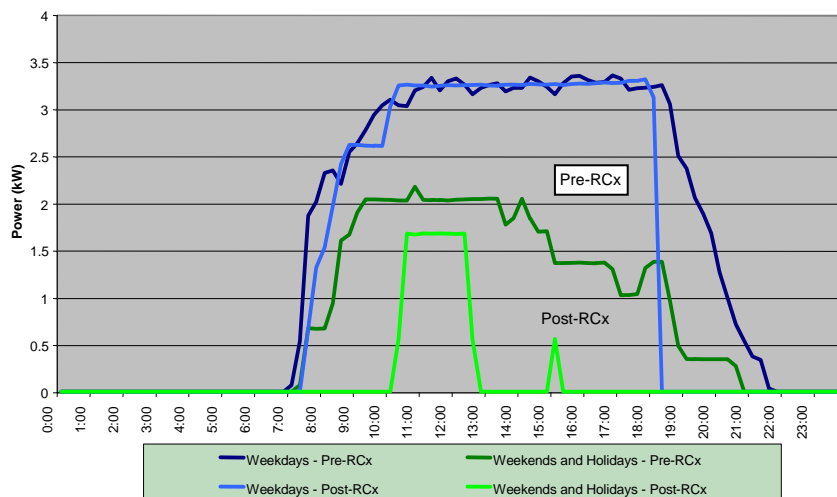
Fluid Cooler Spray Pumps Pre- and Post-RCx Average Daily Load Shapes
