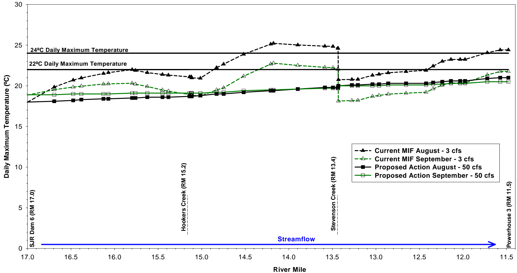
Attachment F-22. San Joaquin River Stevenson Reach (Dam 6 to Powerhouse 3/Redinger Lake) Simulated Daily Maximum Water Temperatures for Proposed Action and Current Minimum Instream Flows (MIF) for the Months of August and September in Above Normal Water Years with Normal Meteorology.
