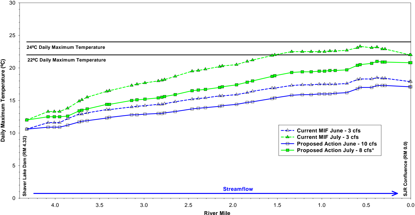
Attachment F-17. Stevenson Creek (Shaver lake Dam to San Joaquin River) Simulated Daily Maximum Water Temperatures for Proposed Action and Minimum Instream Flows (MIF) for the Months of June and July in Above Normal Water Years with Normal Meteorology.
