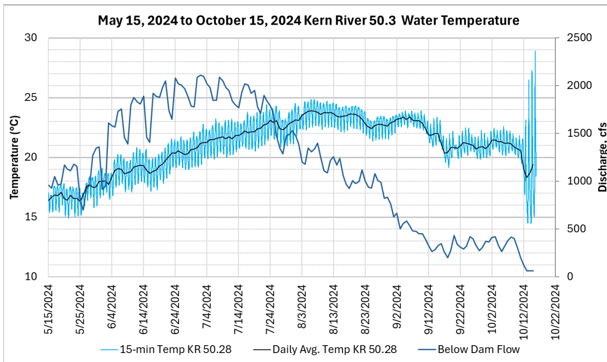
Figure 5-6. Kern River near Lucas Creek, KR 50.3 Water Temperature and Daily Mean Discharge
