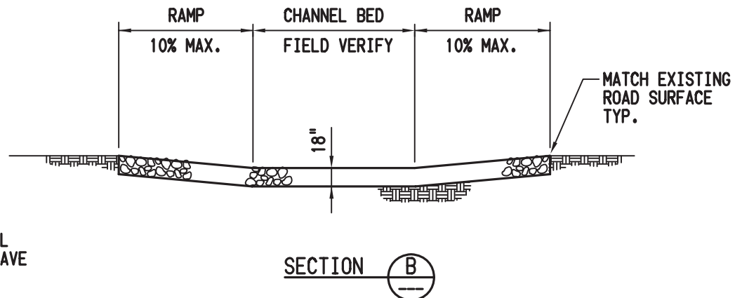
Figure 3.3-2. GROUTED ROCK WET CROSSING TYPICAL INSTALLATION
