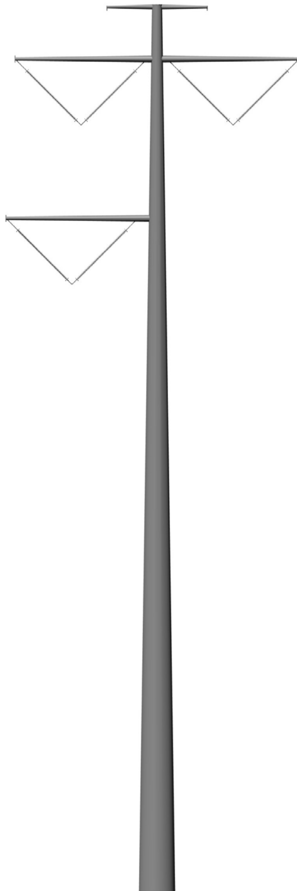
Figure 3.2-3. 500 kV SINGLE-CIRCUIT TUBULAR STEEL POLE
