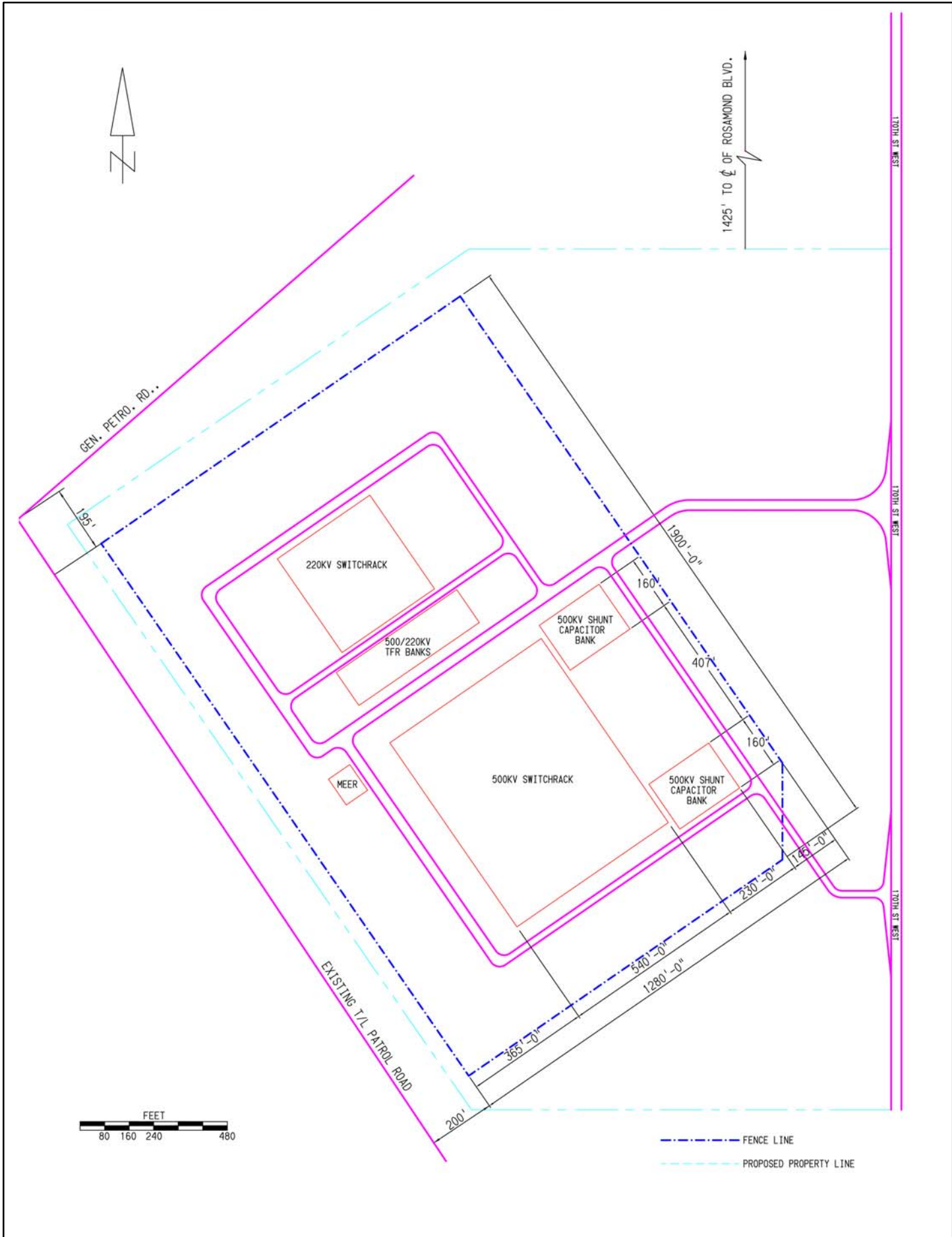
Figure 3.2-12. WHIRLWIND SUBSTATION
