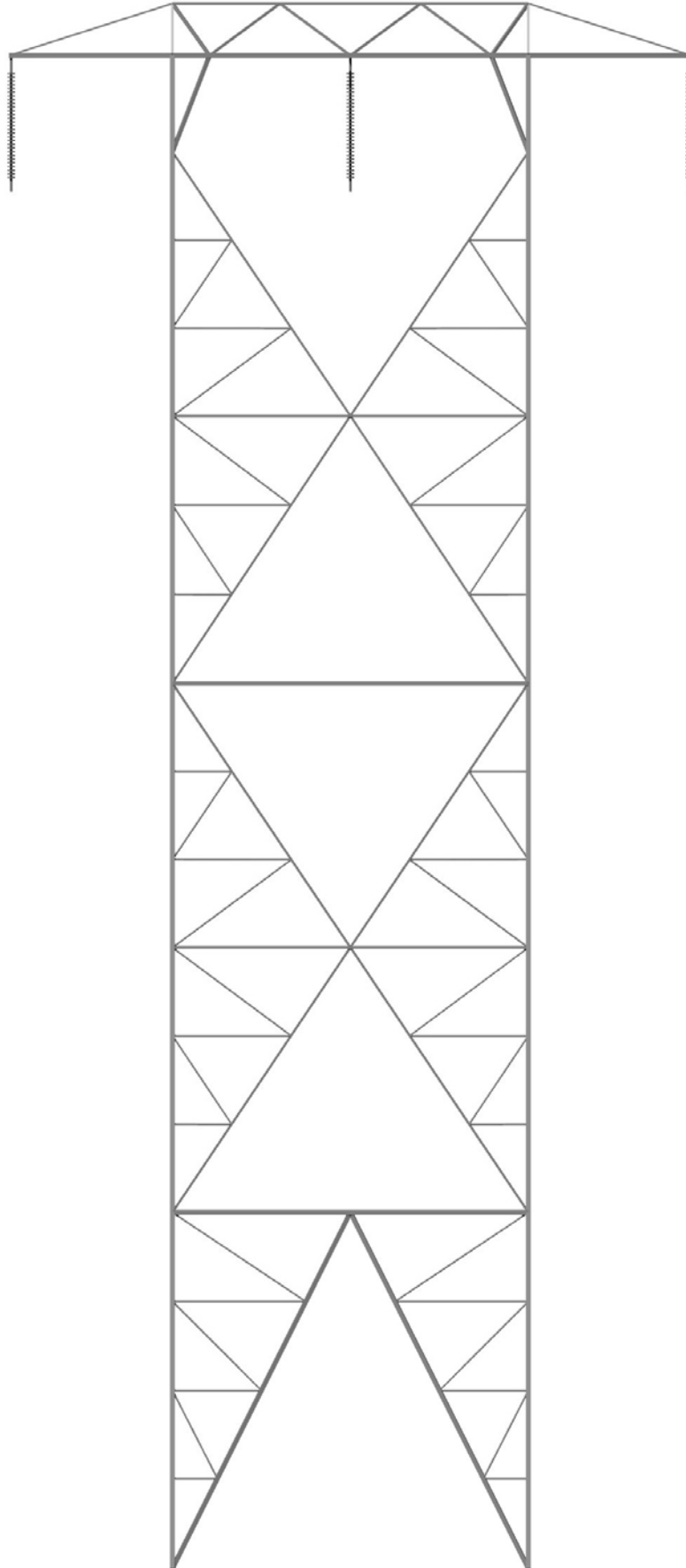
Figure 3.2-1. 220 kV SINGLE-CIRCUIT LATTICE STEEL TOWER
